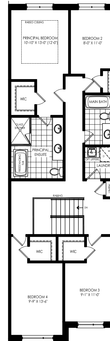
OPTIONAL UPPER FLOOR PLAN EL. 'C-1' W/ 4 BEDROOM PLAN
