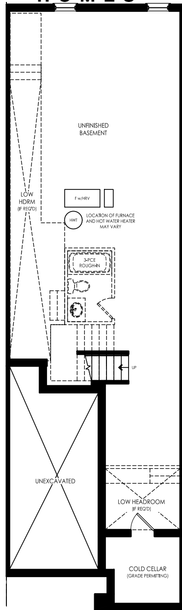
BASEMENT PLAN EL. 'C-1'
