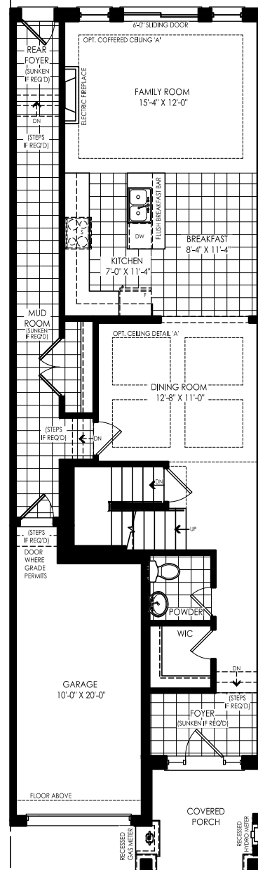
MAIN FLOOR PLAN EL. 'C'
